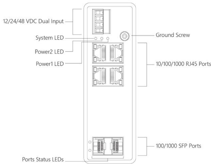
SISTG1040-242-LRT Front Panel
