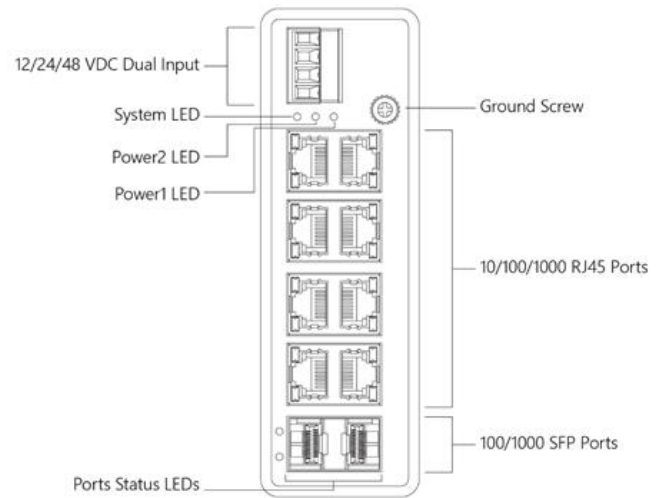
SISTG1040-282-LRT Front Panel
